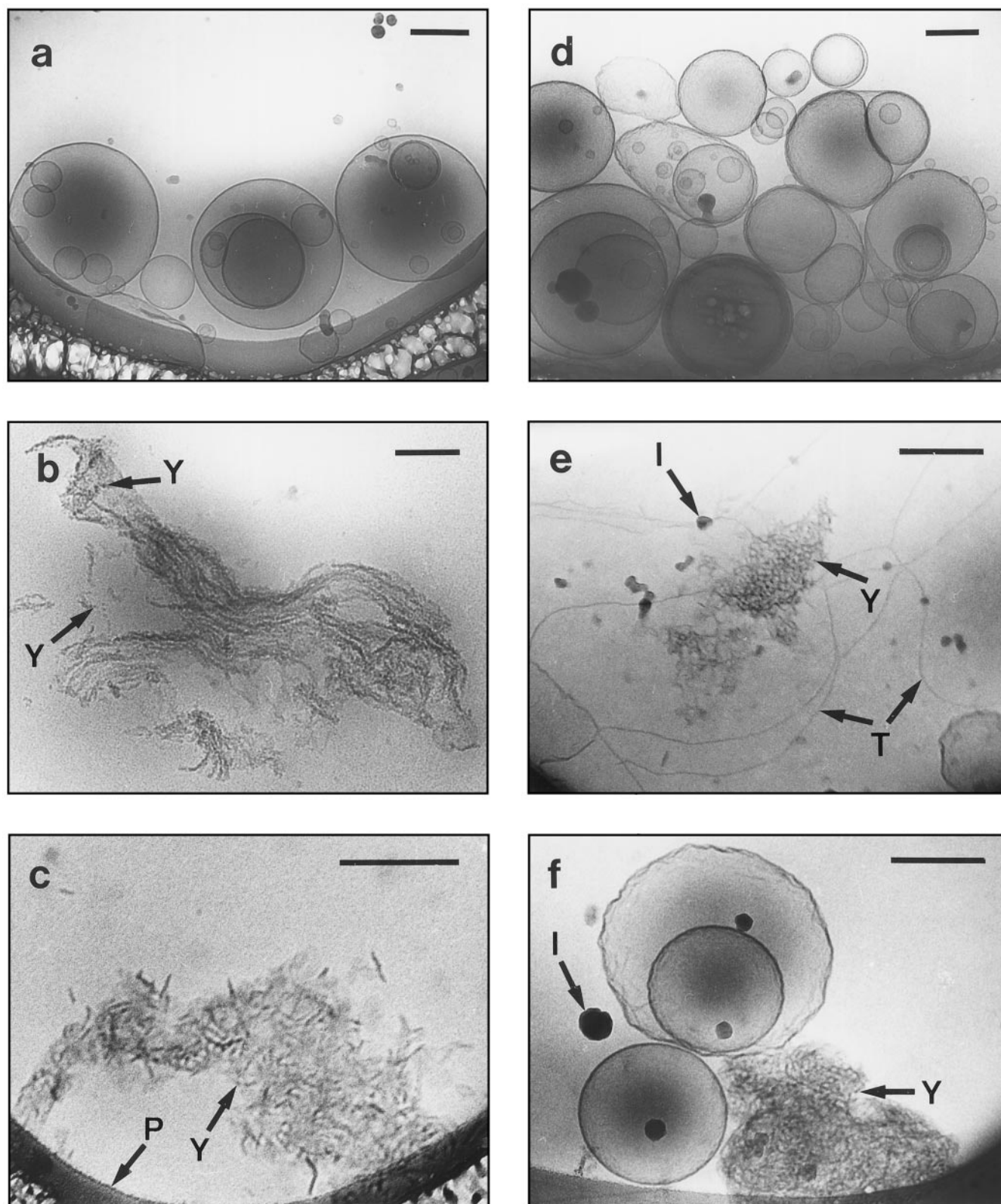
FIGURE 6 Micrographs obtained from (a and d) FATMLV of pure DPPC and (b, c, e, and f) DPPC/nisin samples ( R = 0.2 ). The micrographs a–c were obtained from samples frozen from the gel phase (25°C), whereas d–f were obtained from the fluid phase (50°C). Y indicates some dense globular particles, T indicates thread-like aggregates, P indicates the edge of the polymer support, and I indicates ice crystals deposited on the surface of the sample after vitrification. The bar length corresponds to 200 nm.
